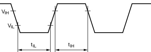
Figure 23.3 Input Timing
